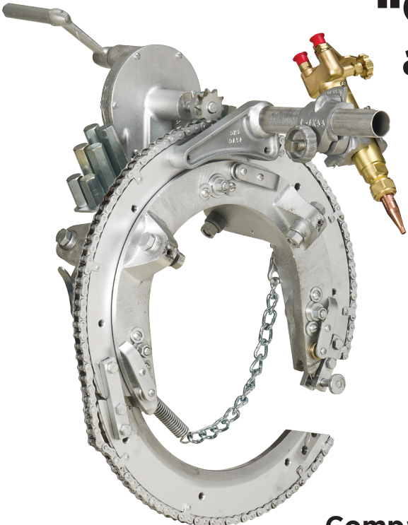
Compact* Model 200C
